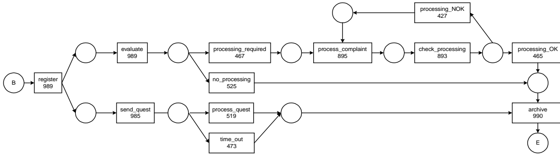
Fig. 6. The WF-net as induced by Little Thumb.
