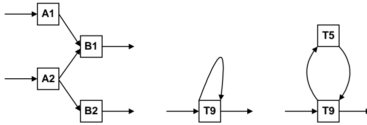
Fig. 3. An overview of the types of dependency relations not recognized by the first version of mining rule 1: (i) complex interconnected structures, (ii) recursion, and (iii) short loops.
