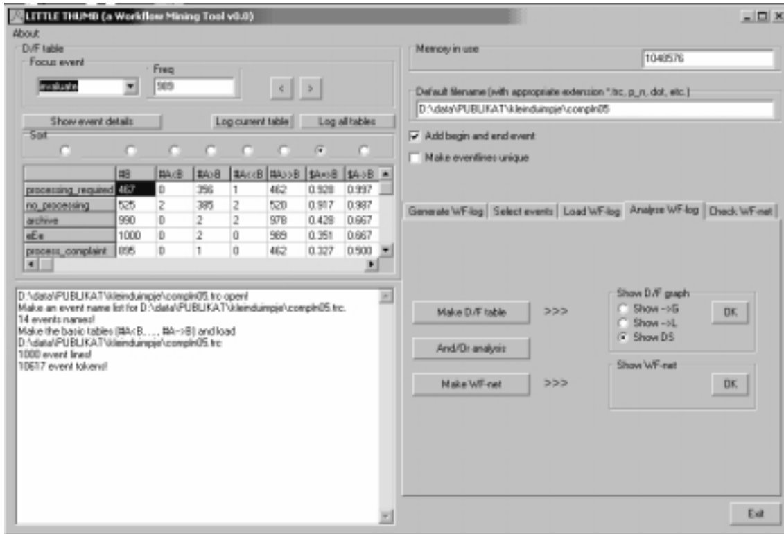
Fig. 4. A screenshot of Little Thumb.
