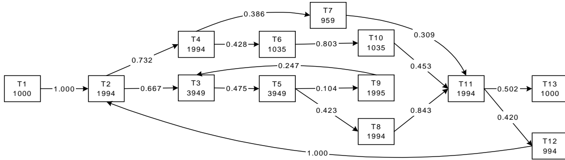
Fig. 2. The extracted D/F-graph based on heuristic rule 1.
