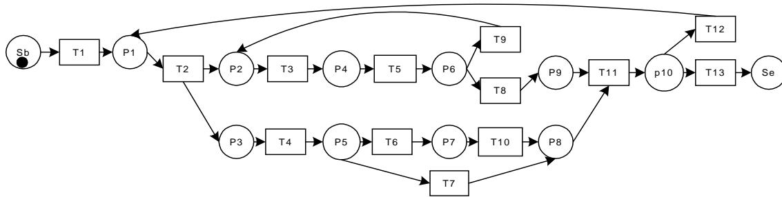
Fig. 1. Example of a workflow process modeled as a Petri net.
