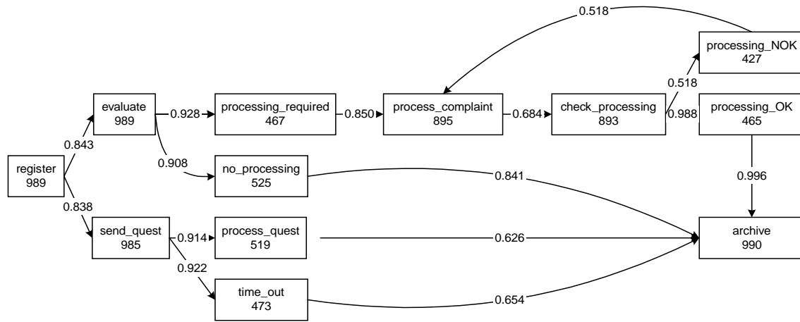
Fig. 5. The resulting D/F-graph of Little Thumb.
